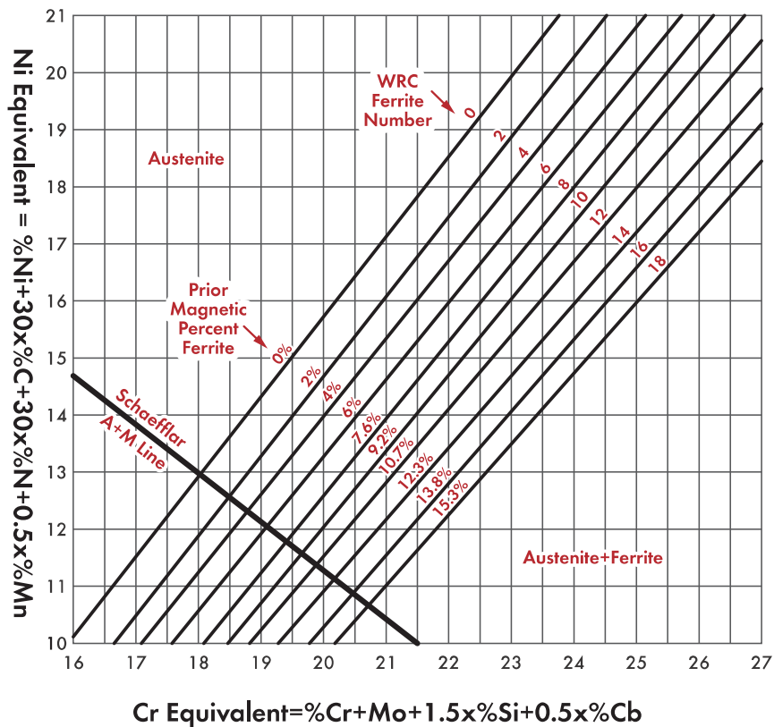
Fig. 2 DeLong's diagram
