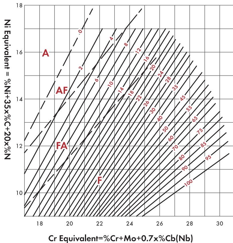
Fig. 3 WRC diagram (1992)
