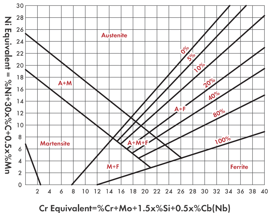
Fig. 1 Schaeffler's diagram
